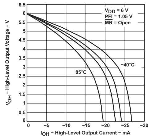
Figure 7-7. High-Level Output Voltage vs High-Level Output Current
