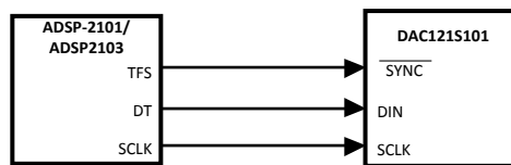
Figure 35. ADSP-2101/2103 Interface
