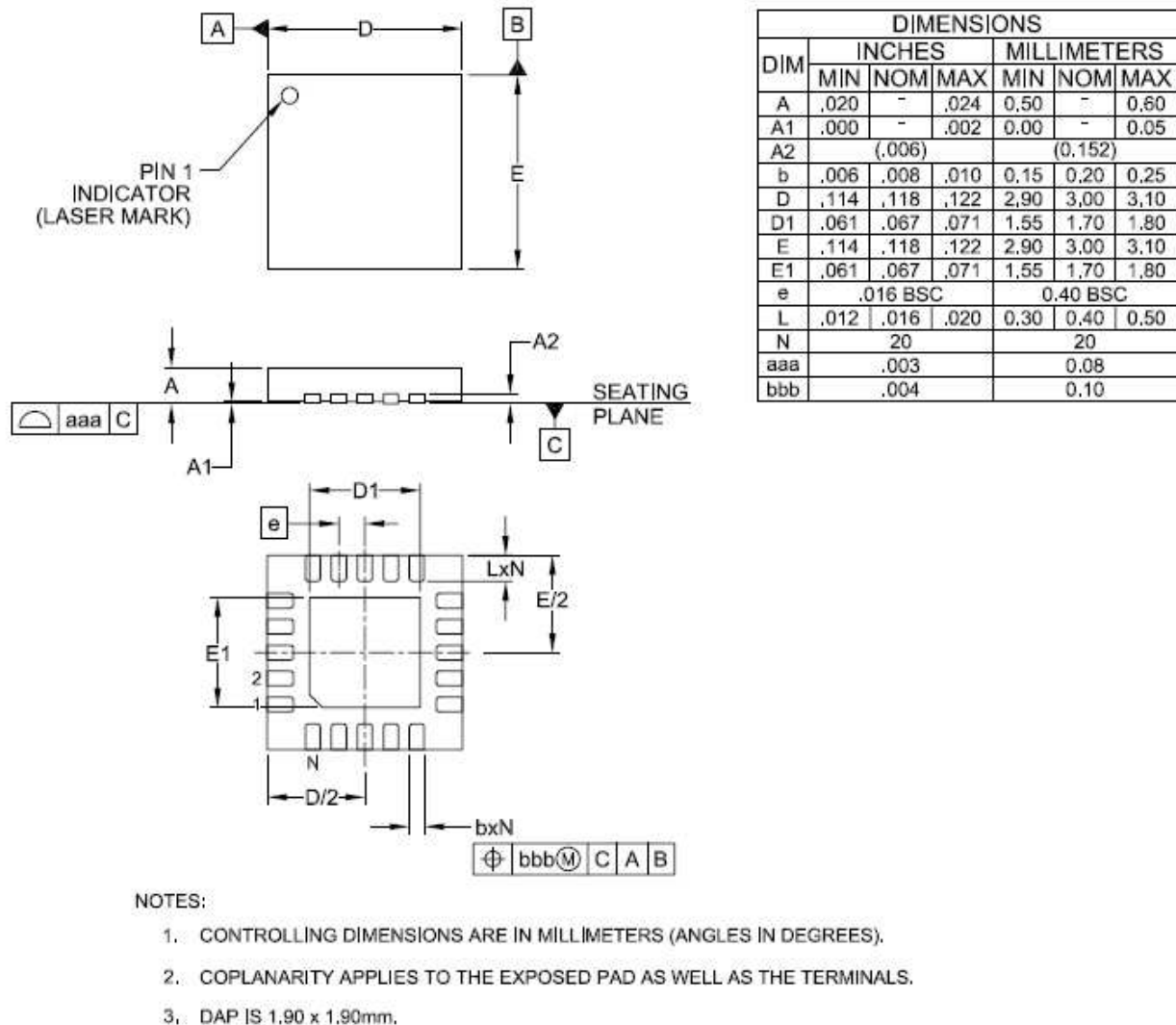
Figure 32: Outline Drawing
