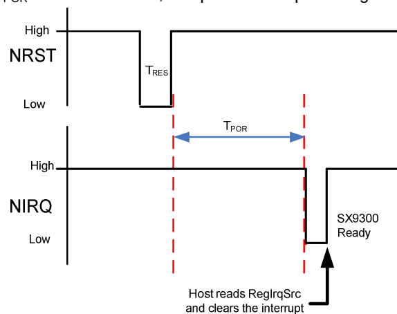
Figure 26: Hardware Reset
