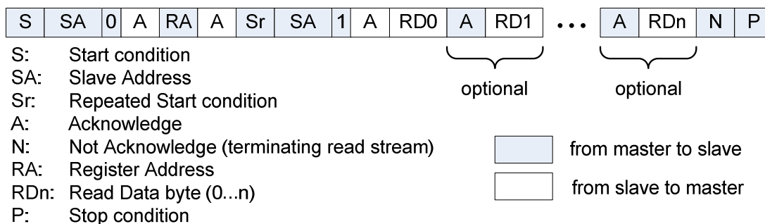
Figure 24: I2C Read
