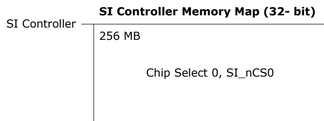
FIGURE 3-17: SI BOOT CONTROLLER MEMORY MAP IN 32-BIT MODE
