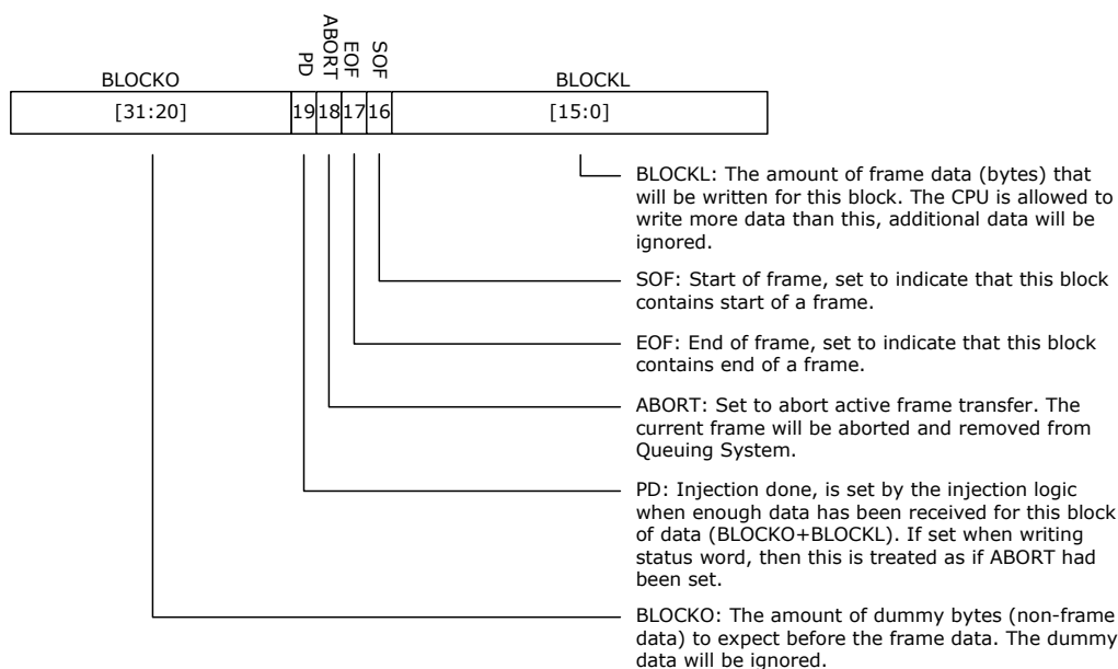
FIGURE 3-15: INJECTION STATUS WORD ENCODING
