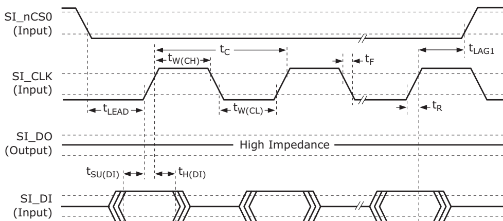
FIGURE 6-4: SI INPUT DATA TIMING DIAGRAM FOR SLAVE MODE
