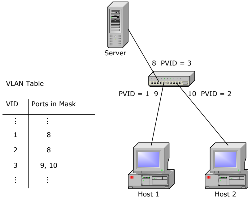
FIGURE 4-4: ASYMMETRIC VLANS
