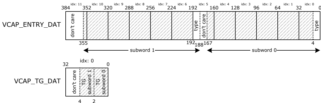
FIGURE 2-24: ENTRY LAYOUT IN REGISTER USING SUBWORDS EXAMPLE
