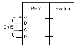
FIGURE 2-11: CONNECTOR LOOPBACK
