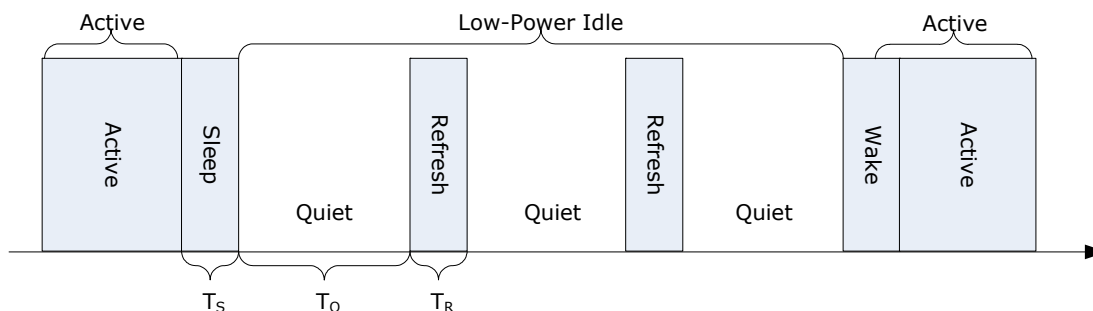
FIGURE 2-5: LOW POWER IDLE OPERATION
