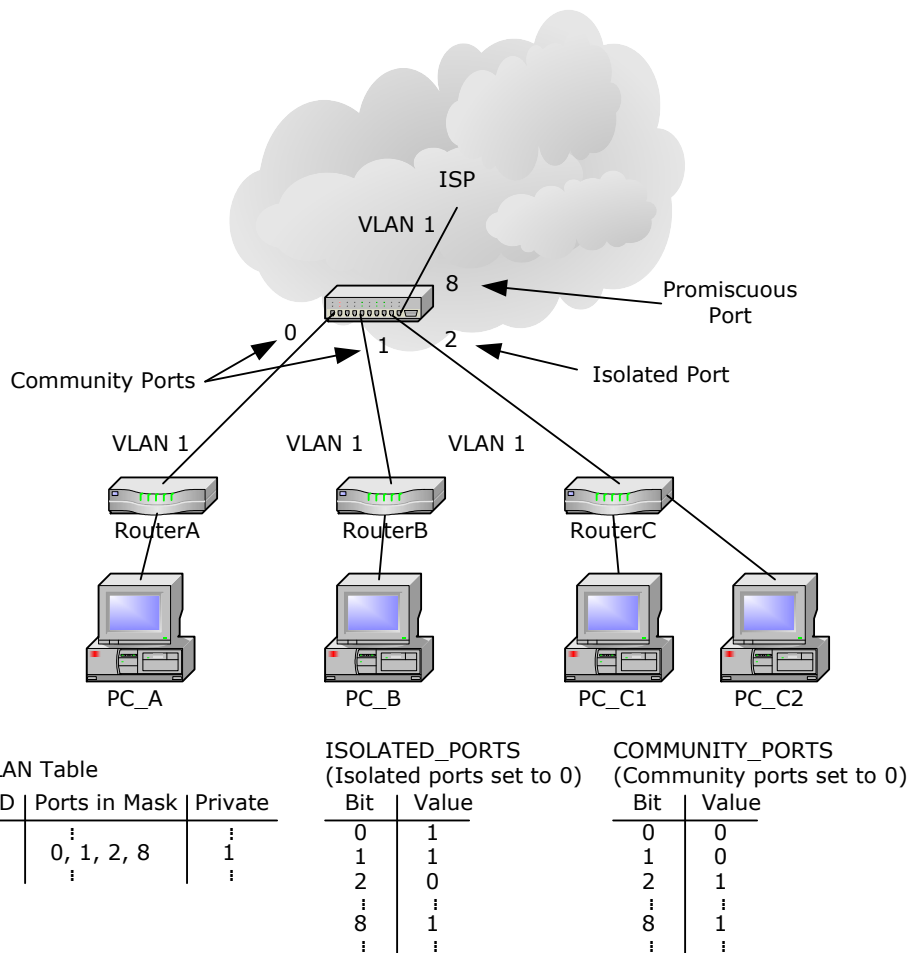
FIGURE 4-2: ISP EXAMPLE FOR PRIVATE VLAN
