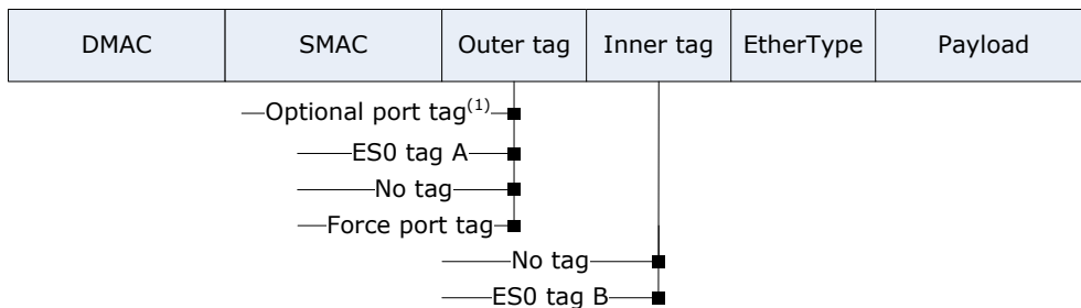
FIGURE 2-36: TAGGING OVERVIEW
