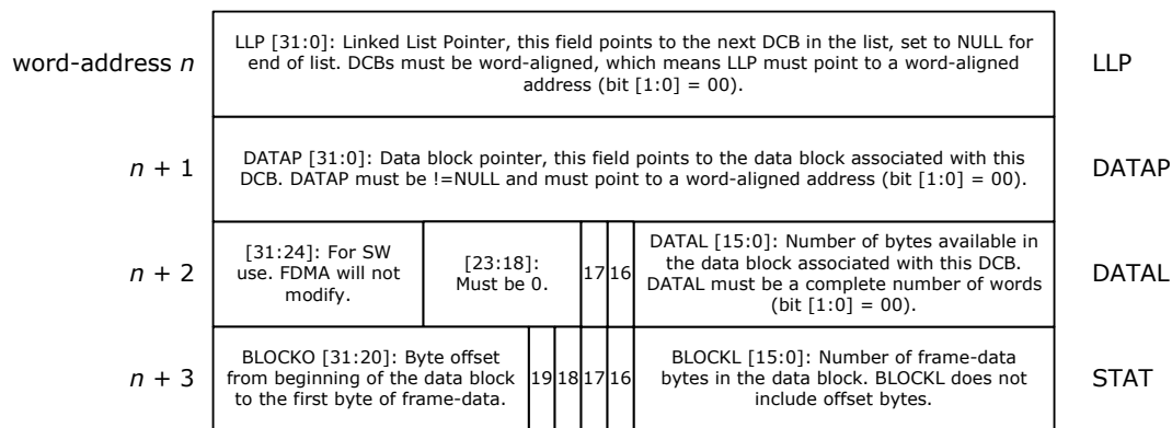
FIGURE 3-11: FDMA DCB LAYOUT
