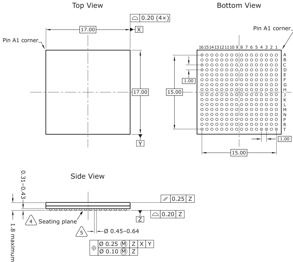
FIGURE 8-1: PACKAGE DRAWING
